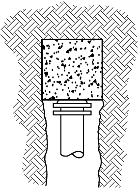
DEAD END THRUST BLOCK
