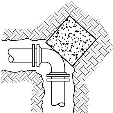
BEND THRUST BLOCK
